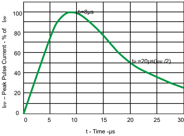
Fig 1. Pulse Waveform
