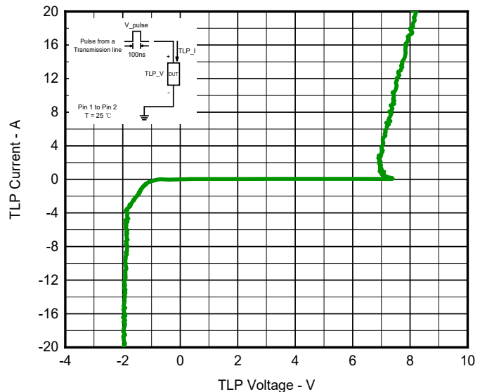
Fig 6. TLP Measurement
