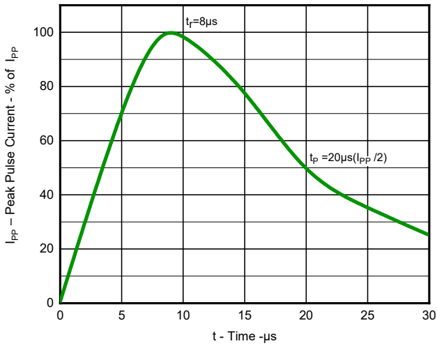
Fig 1. Pulse Waveform(8/20µs)
