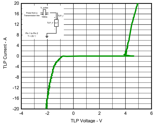
Fig 6. TLP Measurement
