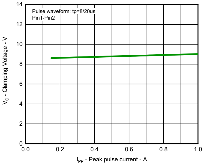
Fig 3. Clamping voltage vs. Peak pulse current
