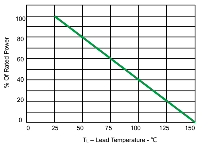
Fig 2.Power Derating Curve
