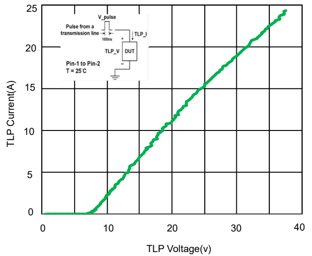
Fig 6. TLP Measurement
