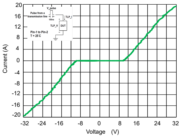
Fig 3. TLP Measurement
