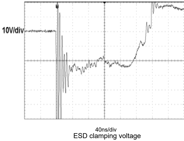
Fig 9. (IEC61000-4-2-8KV contact)
