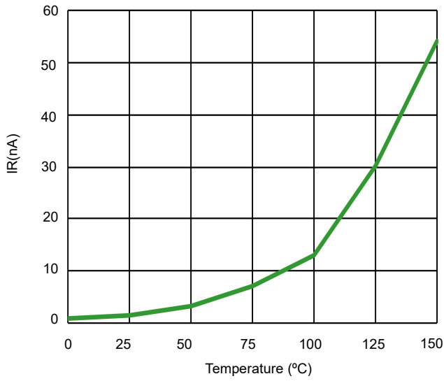
Fig 7. Typical Leakage Current vs. Temperature
