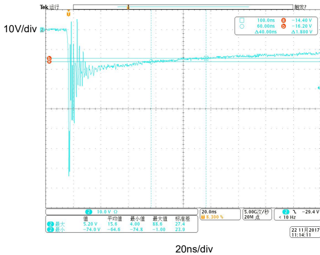
Fig 9. ESD clamping voltage (IEC61000-4-2-8KV contact)
