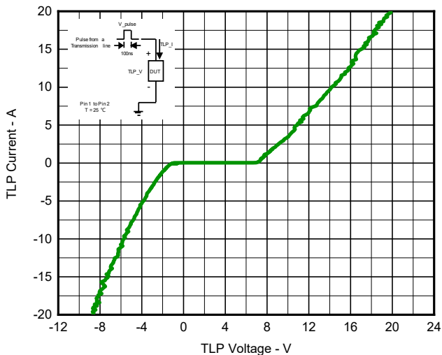
Fig 5. TLP Measurement
