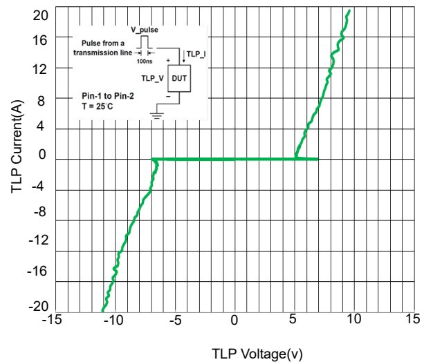
Fig 6. TLP Measurement
