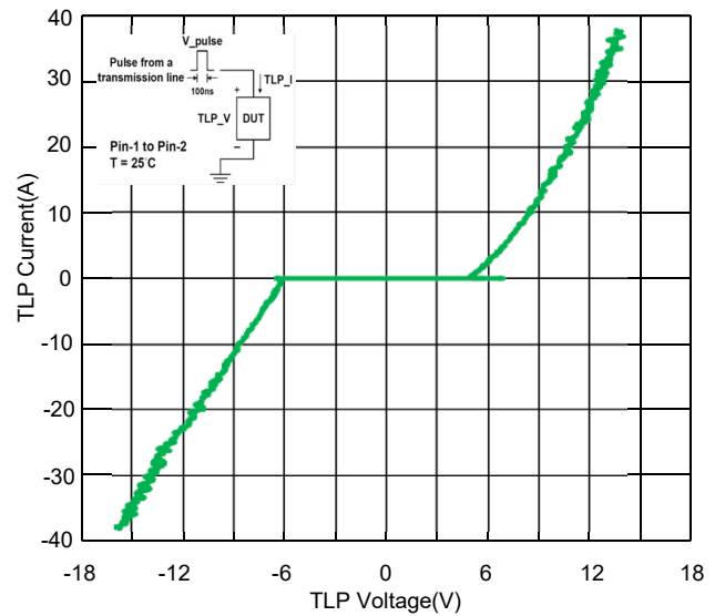
Fig 4. TLP Measurement
