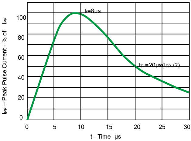
Fig 1. Pulse Waveform
