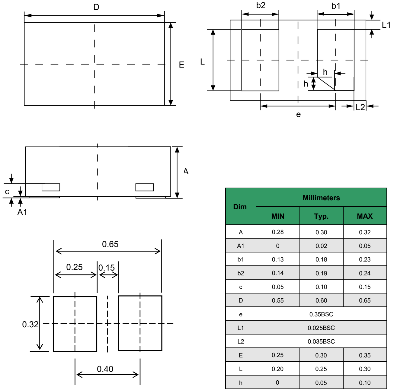
Suggested PCB Layout Unit:mm
