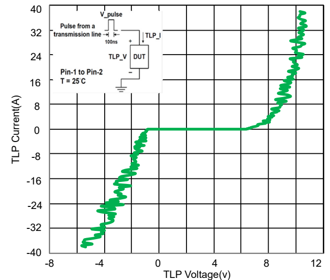
Fig 6. TLP Measurement
