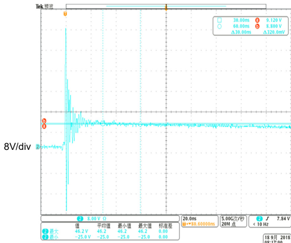
20ns/div ESD clamping voltage (IEC61000-4-2 +8KV contact)
