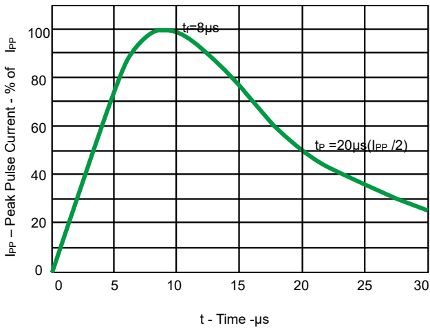
Fig 1. Pulse Waveform
