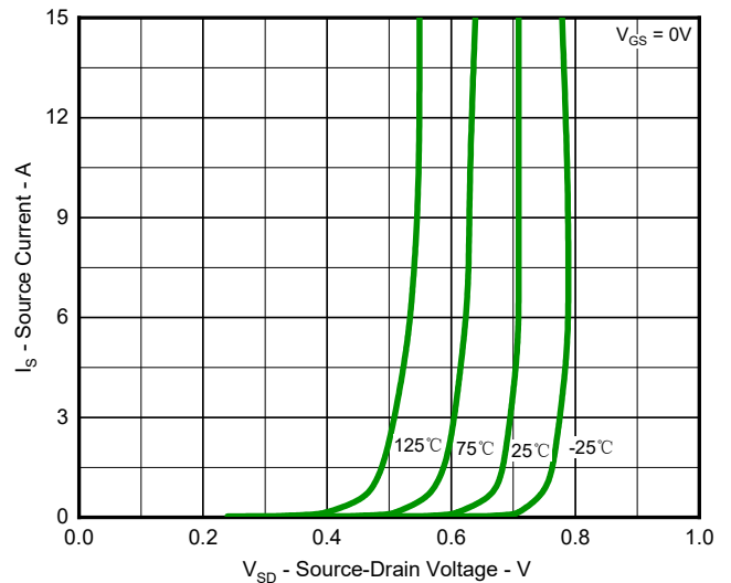
Fig.6 Diode Forward Voltage vs. Current
