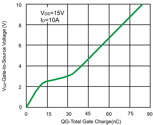
Fig 7. Gate Charge
