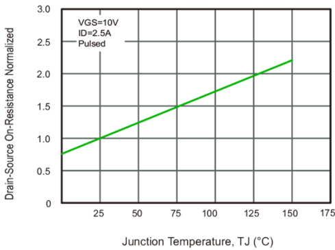
Fig.5 Drain-Source On-Resistance vs. Junction Temperature
