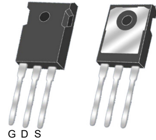
TO-247 (Top View)
