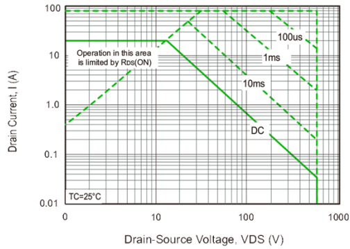
Fig.13 Safe Operating Area
