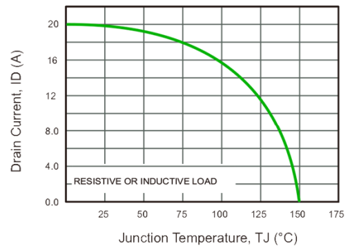
Fig.12 Drain Current vs. Junction Temperature
