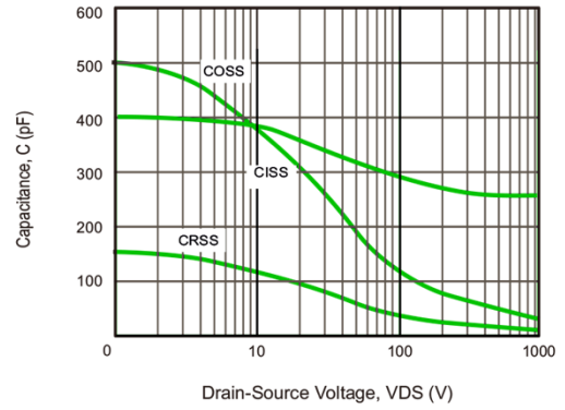
Fig.4 Capacitance Characteristics
