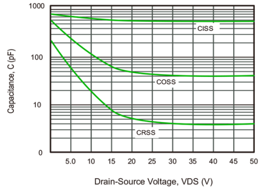
Fig.4 Capacitance Characteristics
