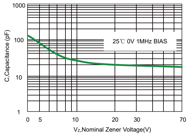
Fig 2. Typical Capacitance
